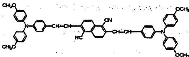
Structural formula (17)-2:
